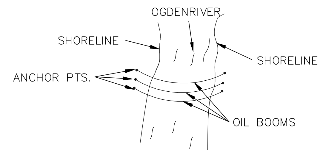
OIL BOOM (TYPICAL)
