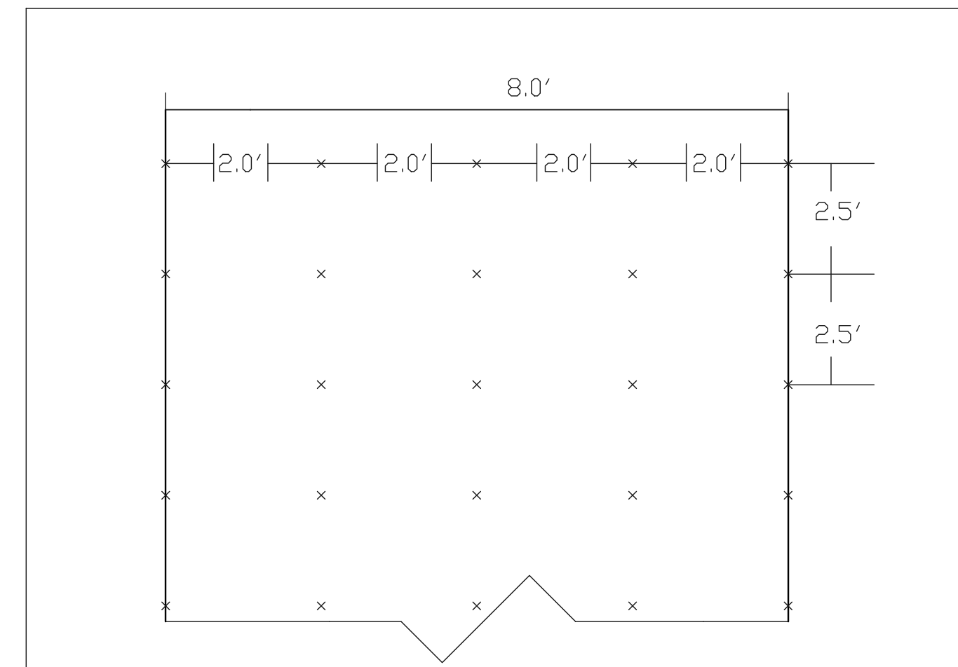
* Denotes Staple Location Figure D- Plan View
