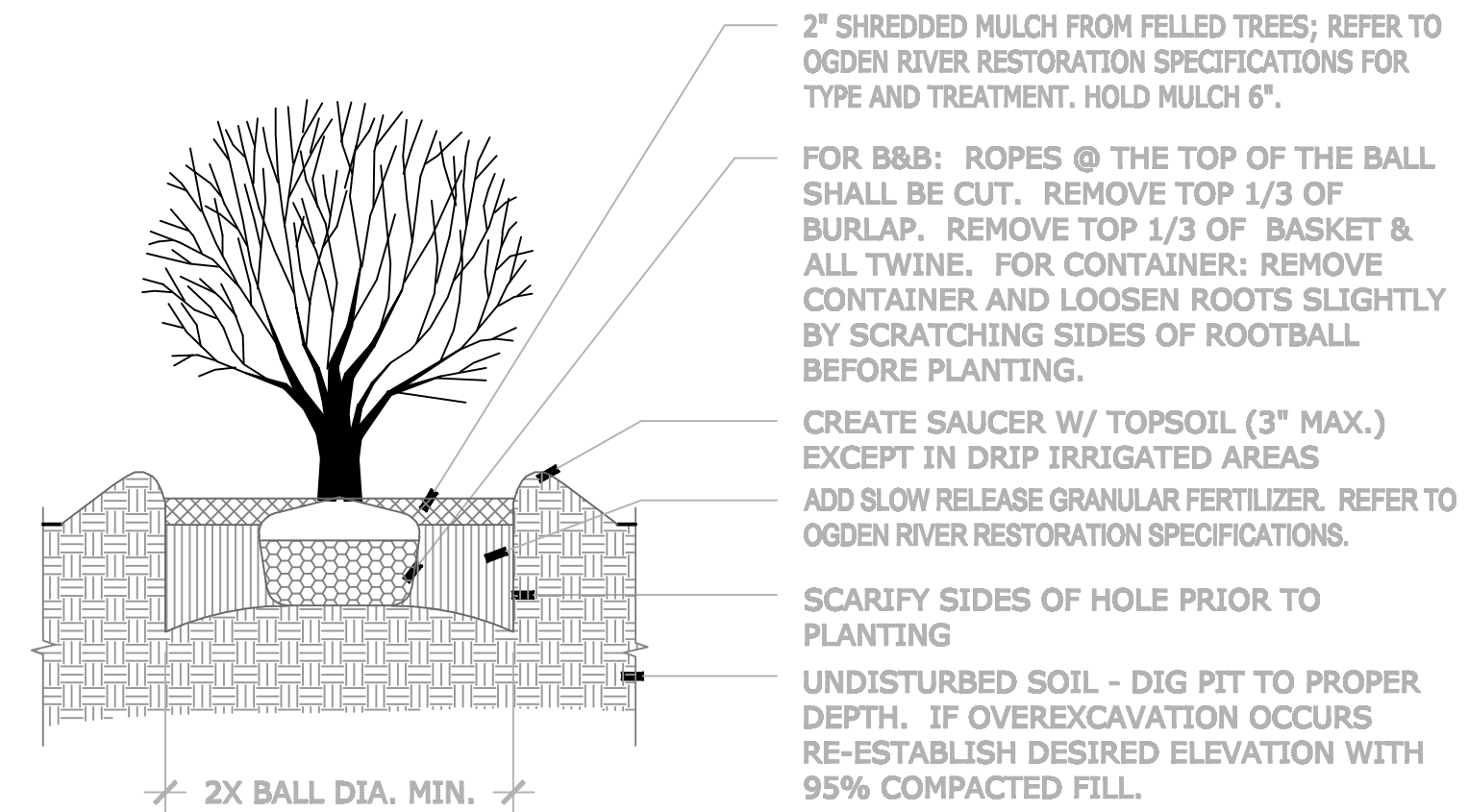
3 SHRUB PLANTING D-4 NTS
