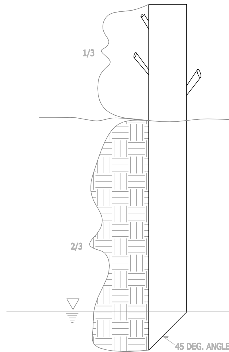
2 STAKE/TREE POLE PLANTING D-4 NTS
