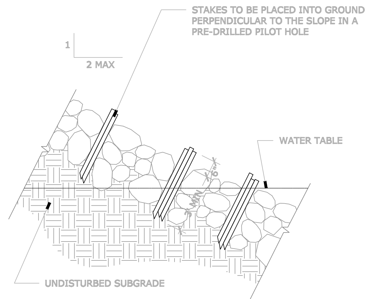
1 POLE STAKING D-4 NTS
